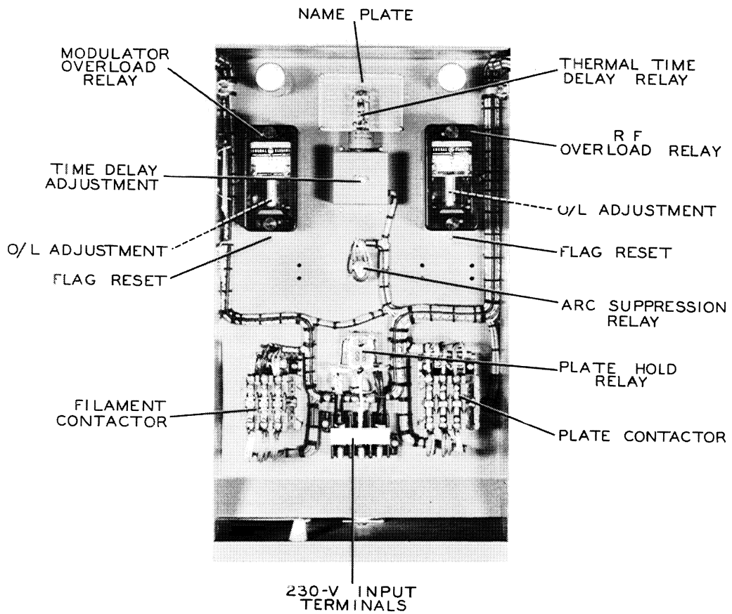
Figure 6-10. Relay Panel Controls
