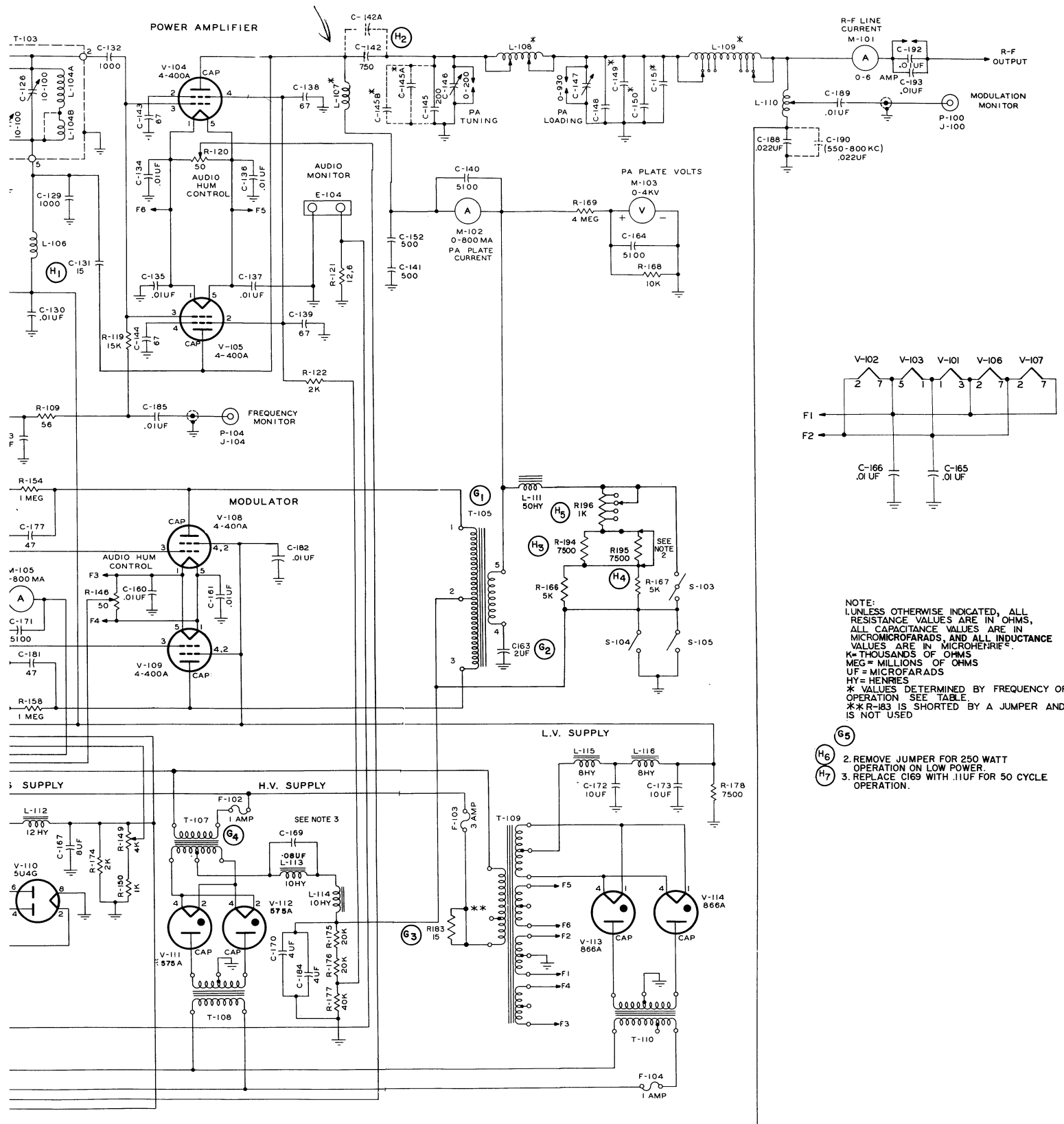
Figure 7-7. Main Schematic
